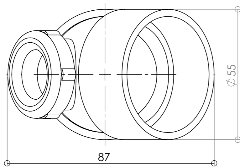
Top View Scale 1:1
