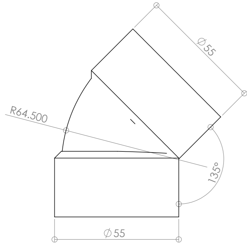
Front View Scale 1:1
