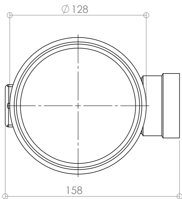
Top View Scale 1:2
