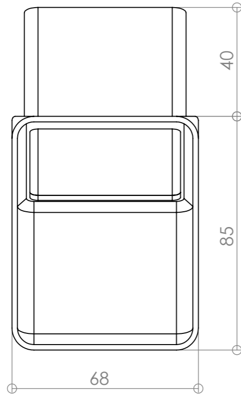
Front View Scale 1:1.4
