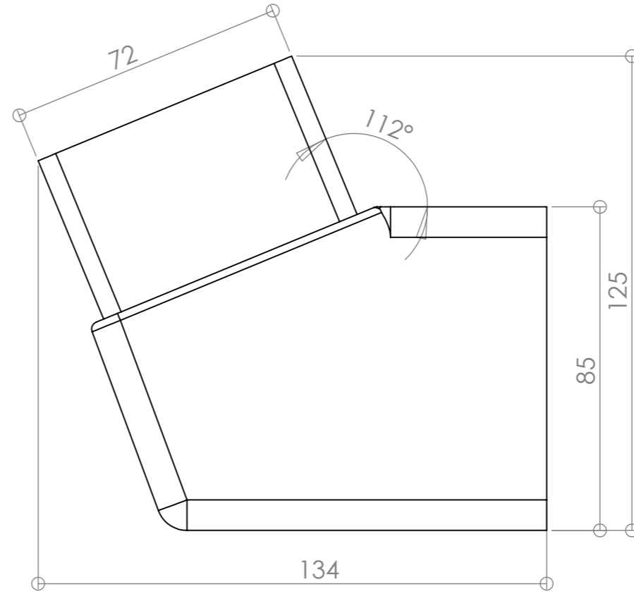
Side View Scale 1:1.4
