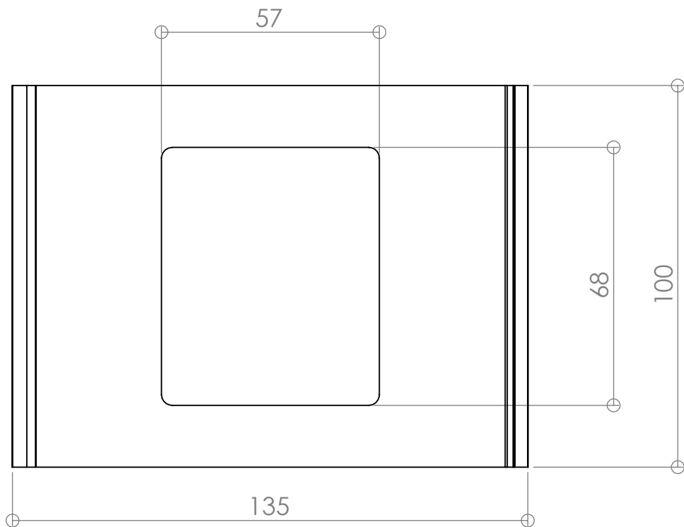
Top View Scale 1:1.4
