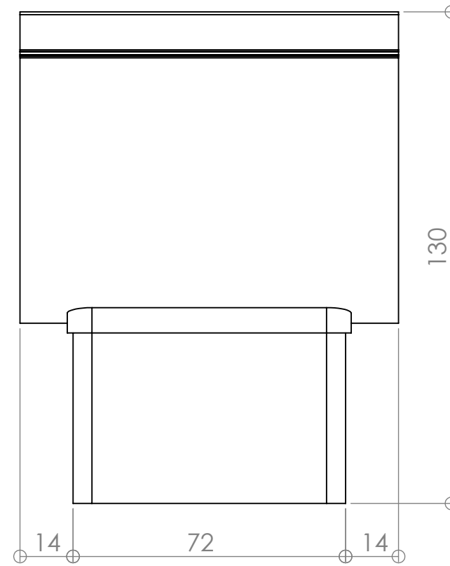
Side View Scale 1:1.4
